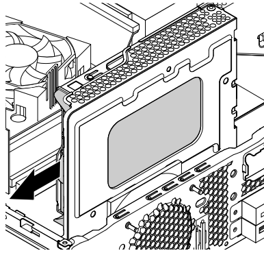
Figure 58. Removing the 3.5-inch storage drive bracket
