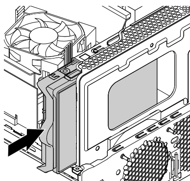
Figure 49. Installing the 3.5-inch storage drive bracket
