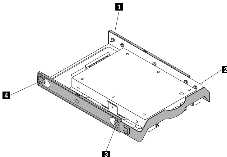
Figure 48. Installing the 2.5-inch storage converter into the 3.5-inch storage drive bracket
