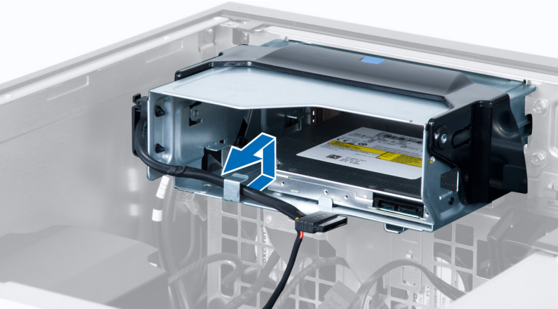
5 Press on the clasp to release the latch holding the cables on the side of the optical-drive cage.
